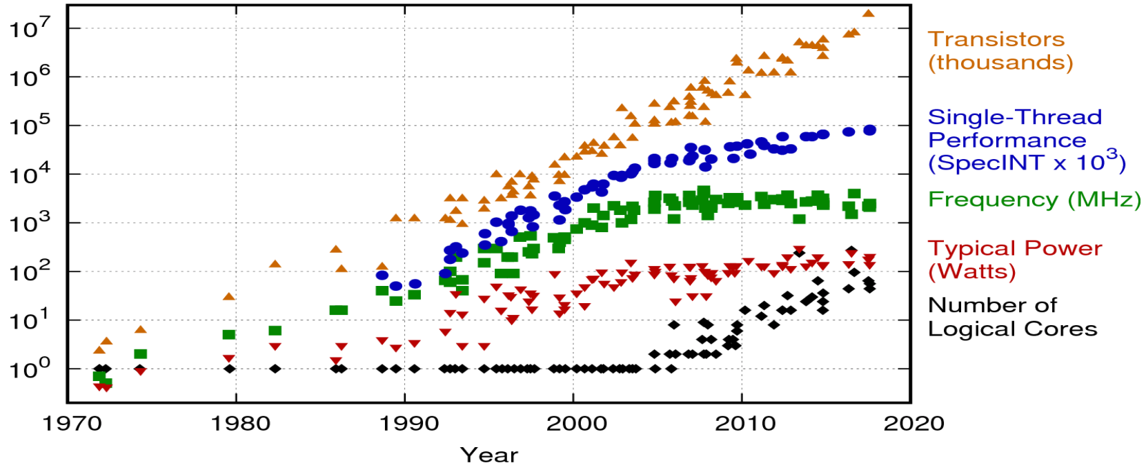
42 Years of Microprocessor Trend Data
